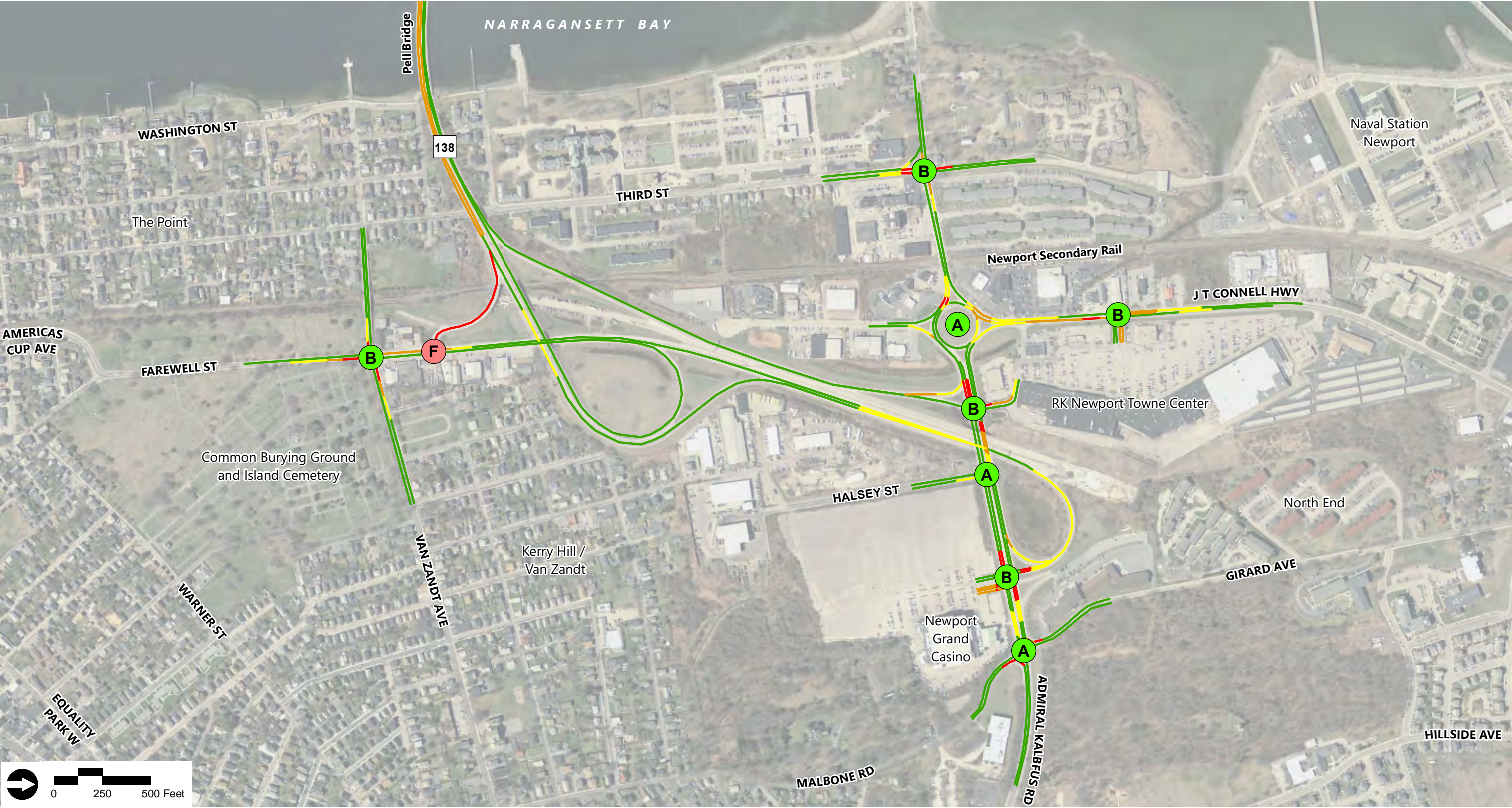
Figure 6 Network Operations Existing Conditions Weekday Morning Reconstruction of the Pell Bridge Approaches Newport/Middletown, Rhode Island
