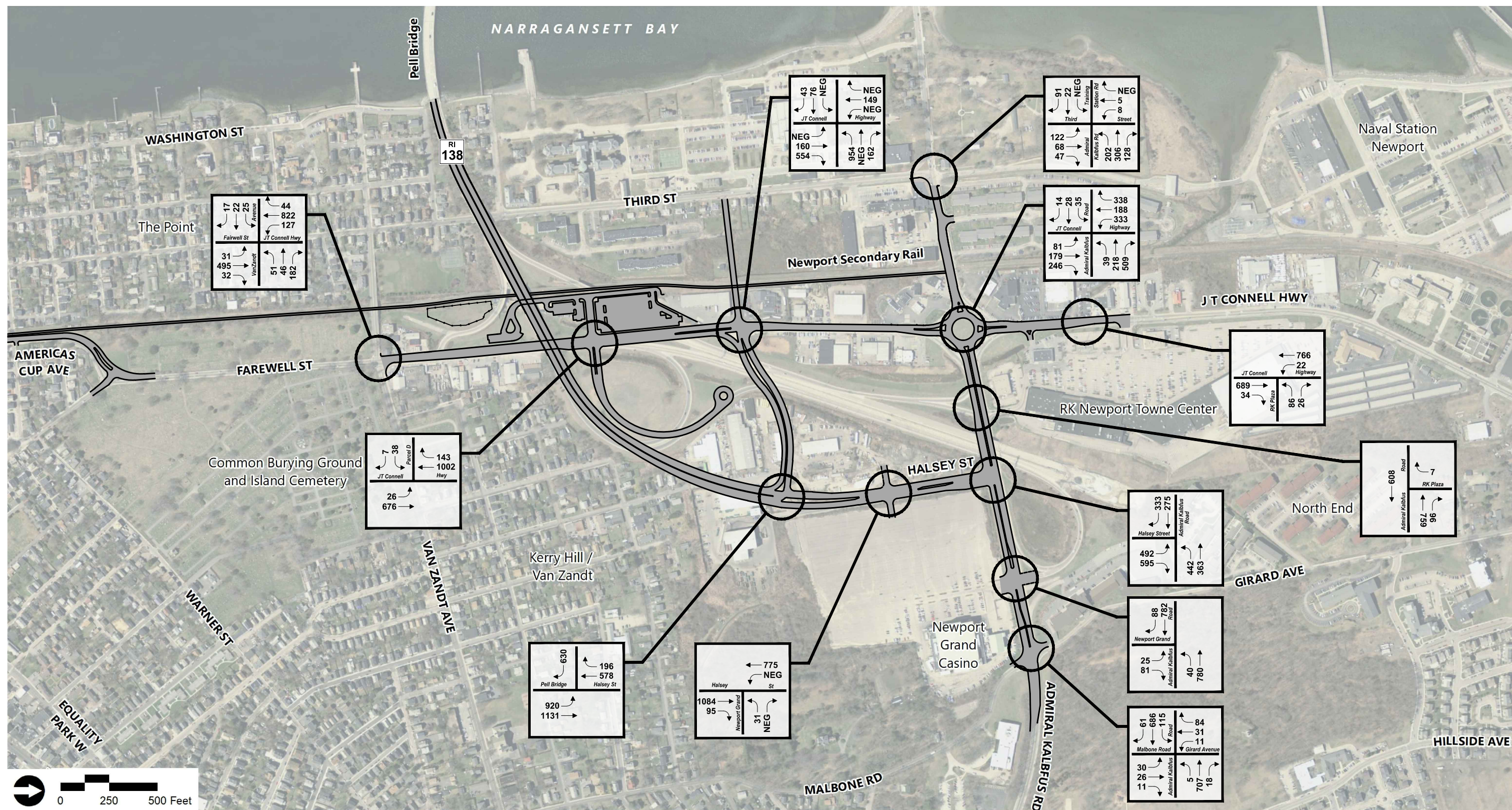
Figure 13 2040 Proposed Action Weekday Morning Peak Hour Traffic Volumes
